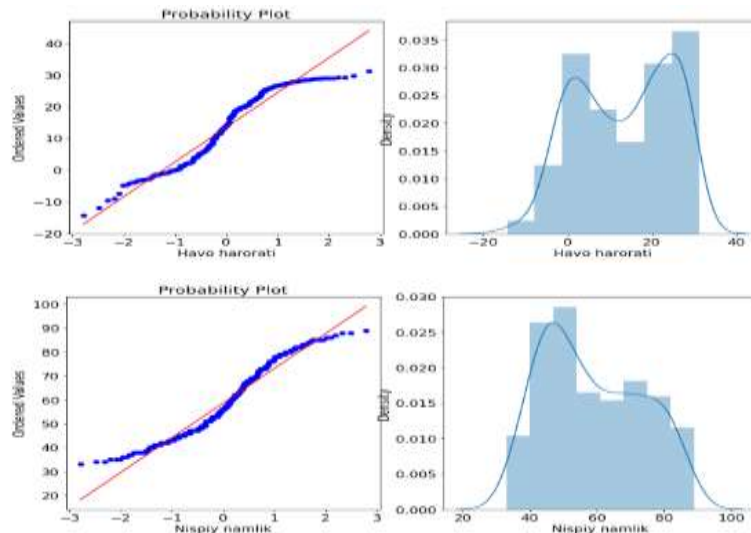
Fig.4. Graph of data distribution in columns.
