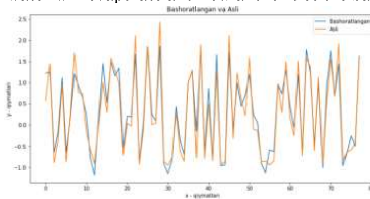
Fig. 6. Conducting a Linear Regression Outcome
