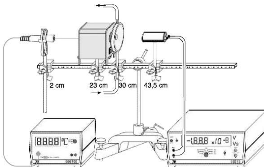
Picture. 1: An experimental device for confirming Stefan-Bolsman's law of thermal radiation.
