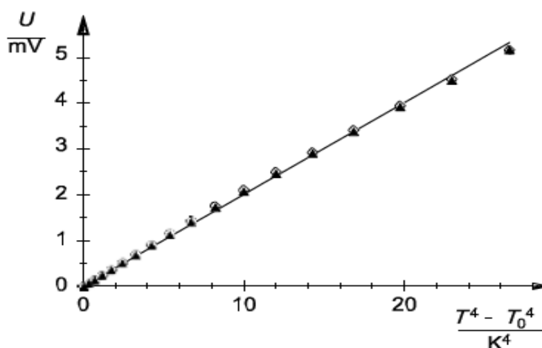
Figure 2: Graph of the output voltage U as a function of T 4 - T 0 4 .
