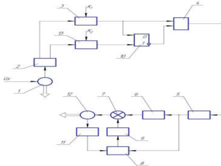
Fig. 5 Coordination of operation of two variable speed drives with negative signal correction for a sensor with low discreteness
