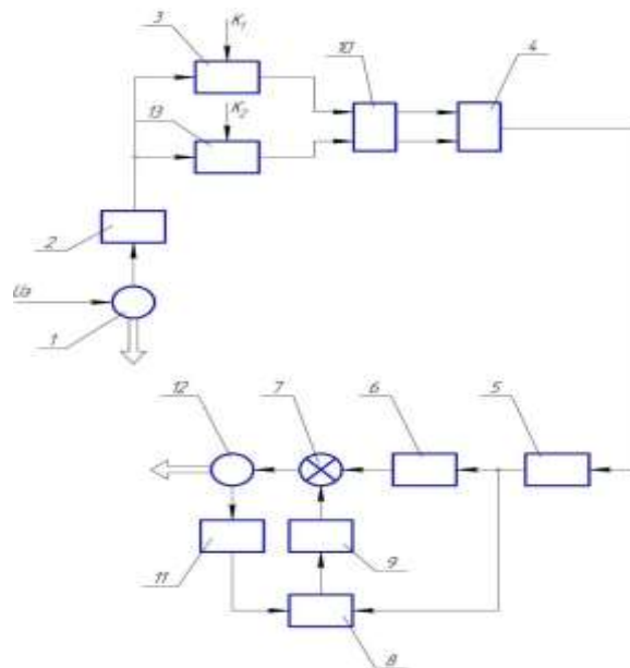
Fig. 8 Coordination of operation of two variable speed drives with positive signal correction for a sensor with high resolution 1, 12- VD; 2, 11- pulse sensor; 3, 13- PFD; 4-element OR; 5- averaging device; 6-PVC; 7- adder; 8- trigger discriminator; 9- filter; 10- BS
