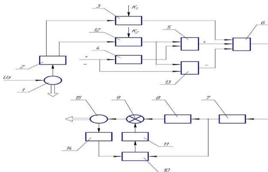
Fig. 3. Coordination of operation of two variable speed drives with signal correction for a sensor with low resolution
