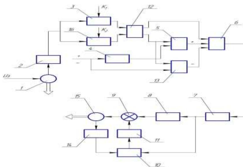
Fig. 4. Coordination of operation of two variable speed drives with signal correction for a sensor with high-resolution
