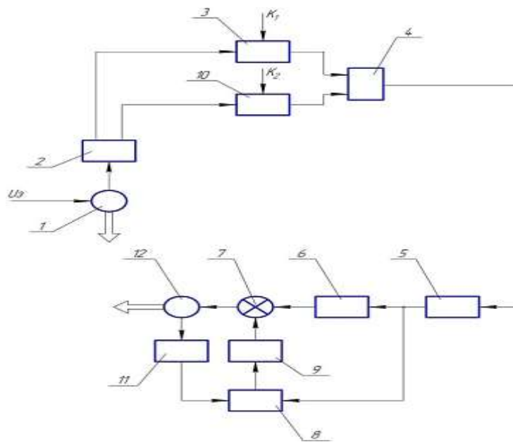
Fig. 7 Coordination of operation of two variable speed drives with positive signal correction for a sensor with low resolution 1, 12- VD; 2, 11- pulse sensor; 3, 10- PFD; 4-element OR; 5- averaging device; 6- PVC; 7-adder; 8-trigger discriminator; 9- filter
