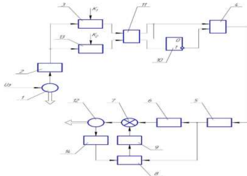
Fig.6 Coordination of operation of two variable speed drives with negative signal correction for a sensor with high resolution
