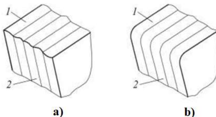
Fig. 2. View of cutting edge of the gun drill
