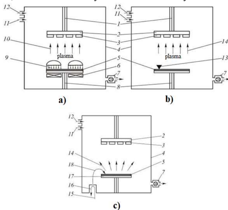
Fig. 3. Schematic diagrams of covering deposition on cutting tool by PVD-methods
