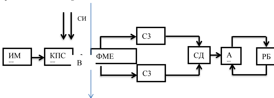
Figure 1 Photomagnetic converter from magnetic field to electric field.
